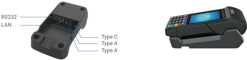
Charging Cradle
